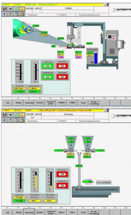
Graphic visualization of underwater pelletizing system and extruder dosing
