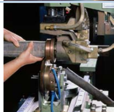
Roll seam
