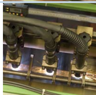
Plasma cutting
